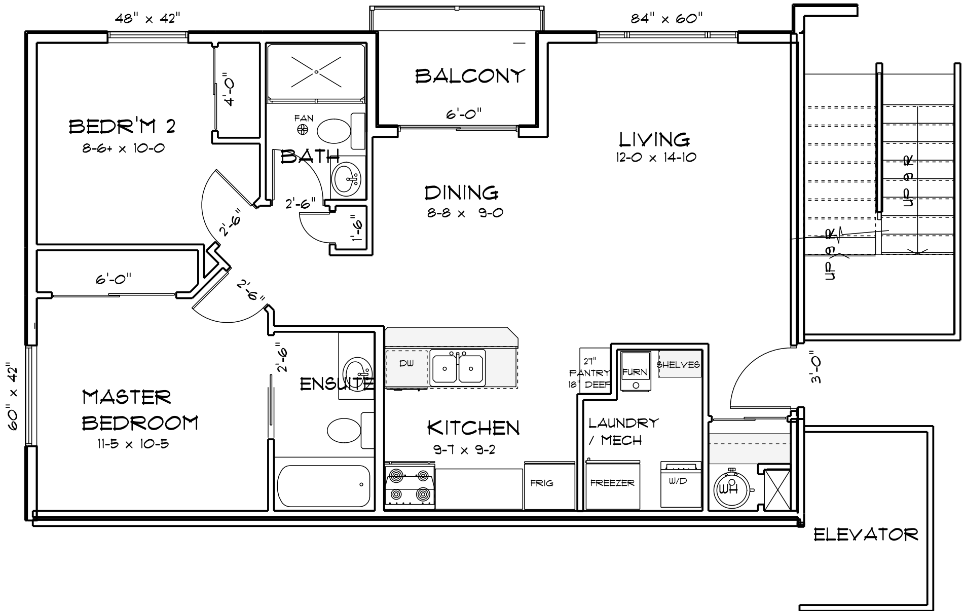
FLOOR PLAN TYPICAL UNIT
